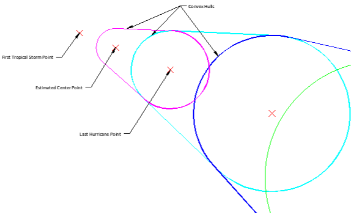
Figure 2: Example of Convex Hulls for Fictional Cyclone
