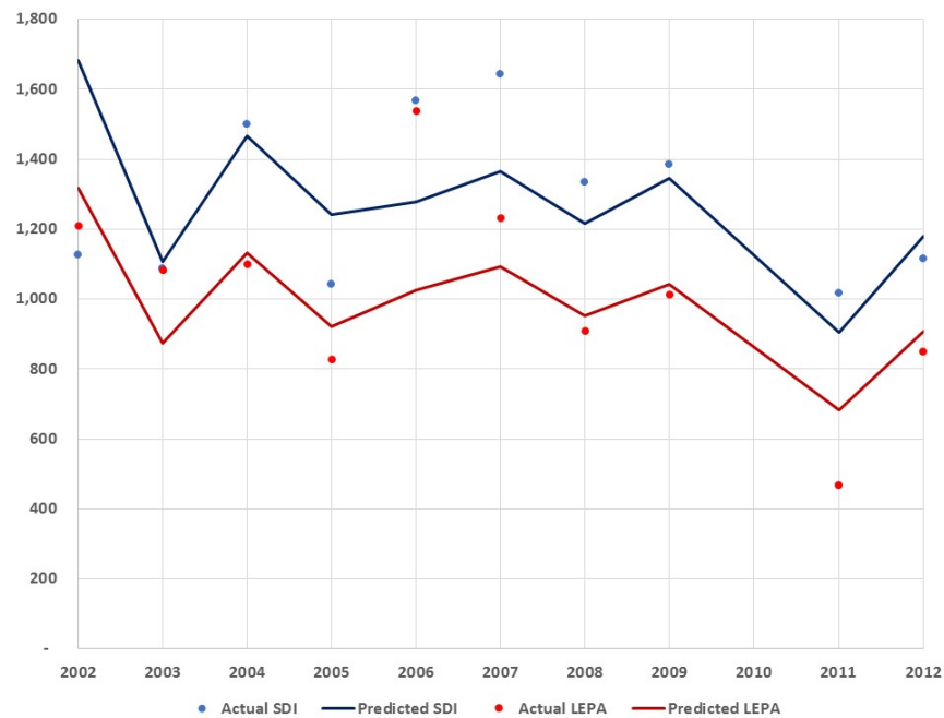
Figure 9. Actual and Predicted Yields – SDI vs. LEPA 2002 - 2012
