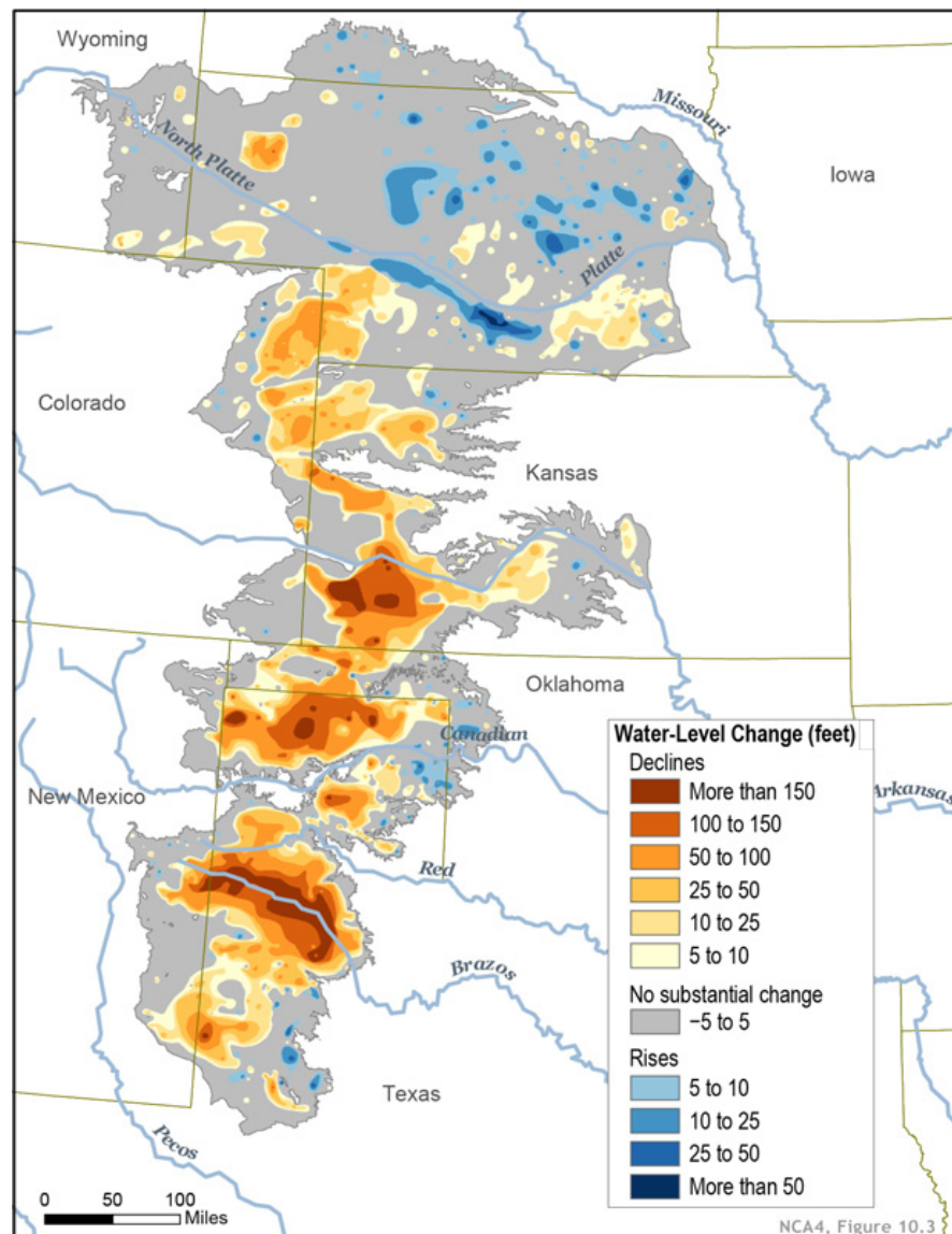
Figure 2. Water-level Changes in the Ogallala Aquifer, 1950-2015
